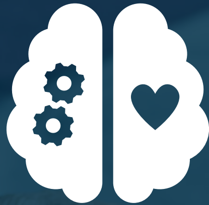
Recommender System
